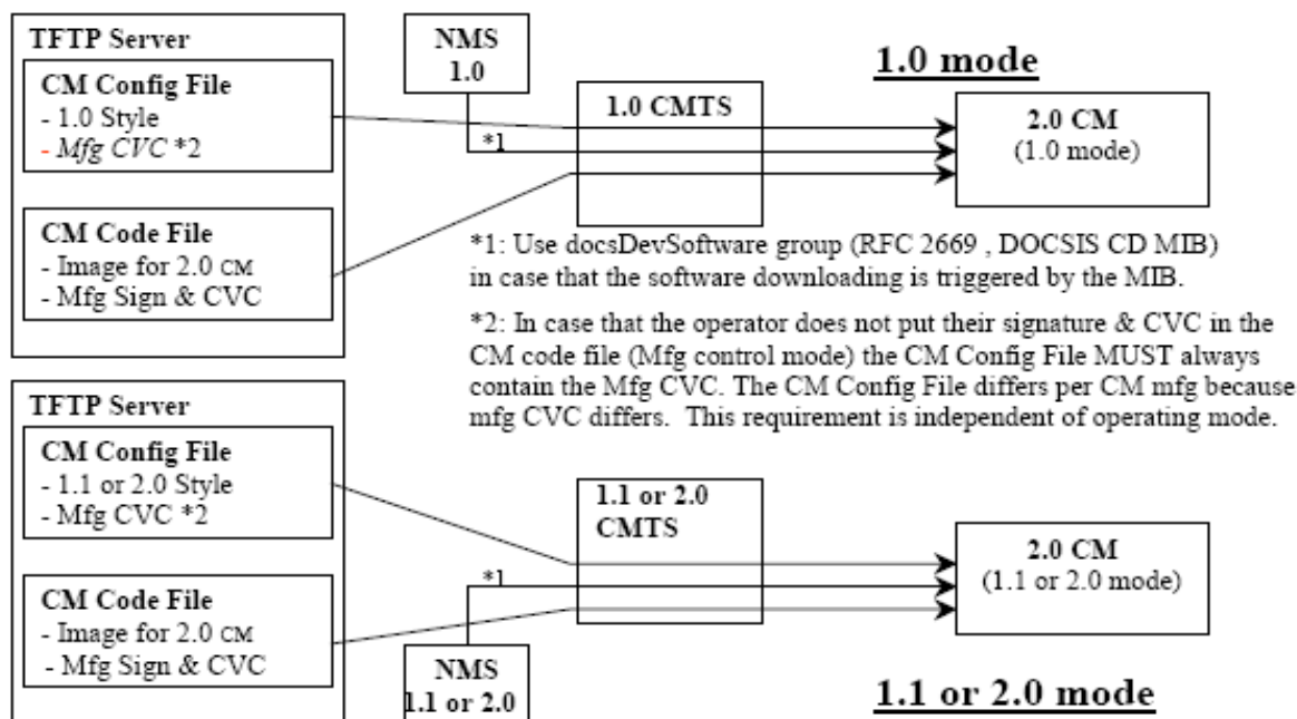
Figure 7-8 - Manufacturer control scheme
