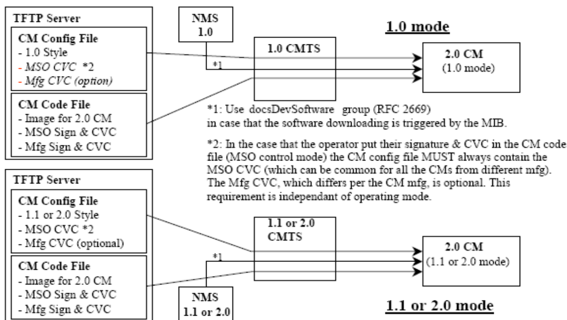
Figure 7-9 - Operator control scheme
