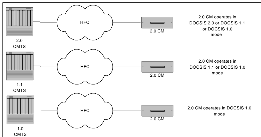
Figure 7-10 - Coexistence (DOCSIS 1.0 mode vs. DOCSIS 1.1 mode vs. DOCSIS 2.0 mode)
