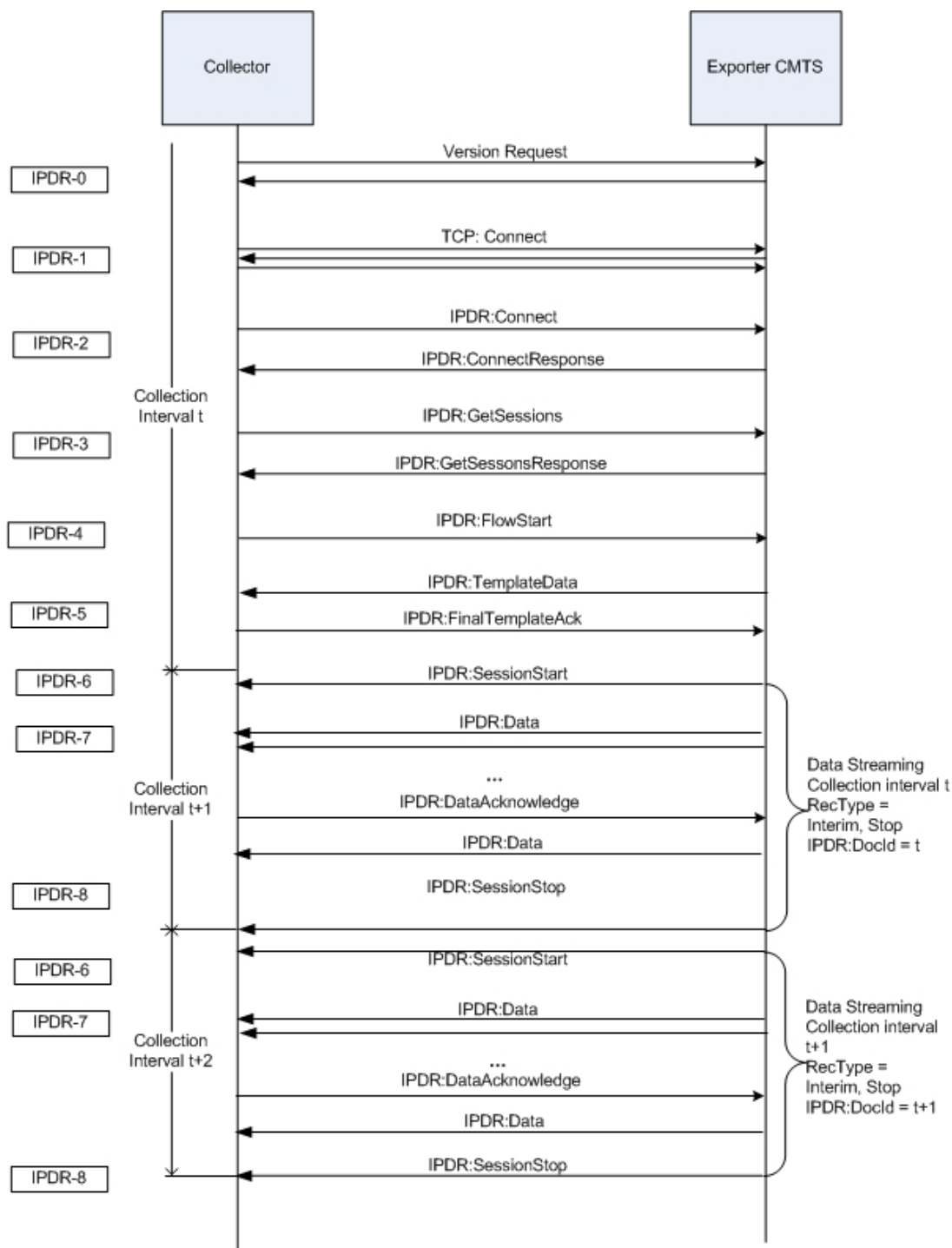
Figure 7-7 - Flow Diagram for DOCSIS Default Streaming Requirements
