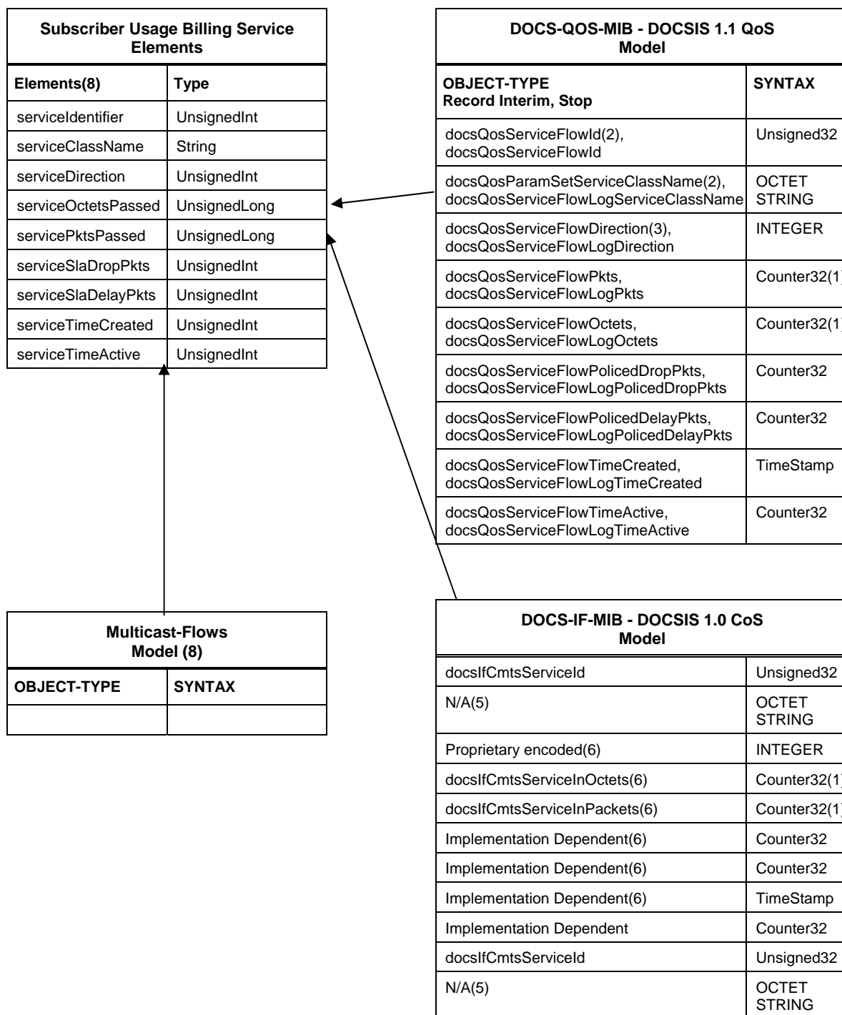
Figure 7–1 - Subscriber Usage Billing Model Mapping to DOCSIS Management Objects
